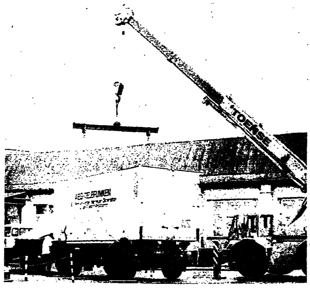
ON THE AIR — Three West German firms have jointly developed a mobile television transmitter for the Federal Post Office, which intends using it for programmes on two national channels. The 10-kilowatt transmitter can be transported in a container to any part of the country, and can be used to keep transmissions on the air while repair or maintenance work is being done to the main transmitters. The portable transmitter also has a highly-sensitive sound volume capacity.
